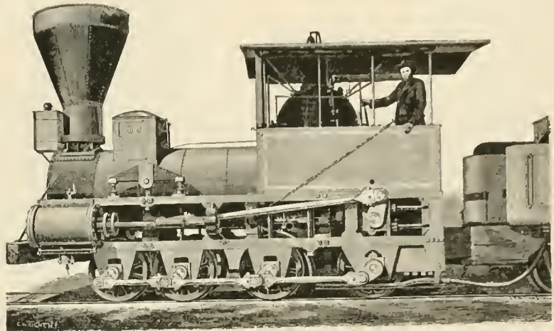
THE MUD DIGGER
